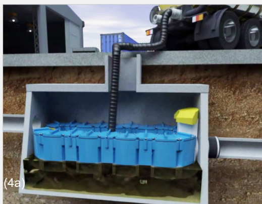
Sediment is removed with a standard vacuum truck.
